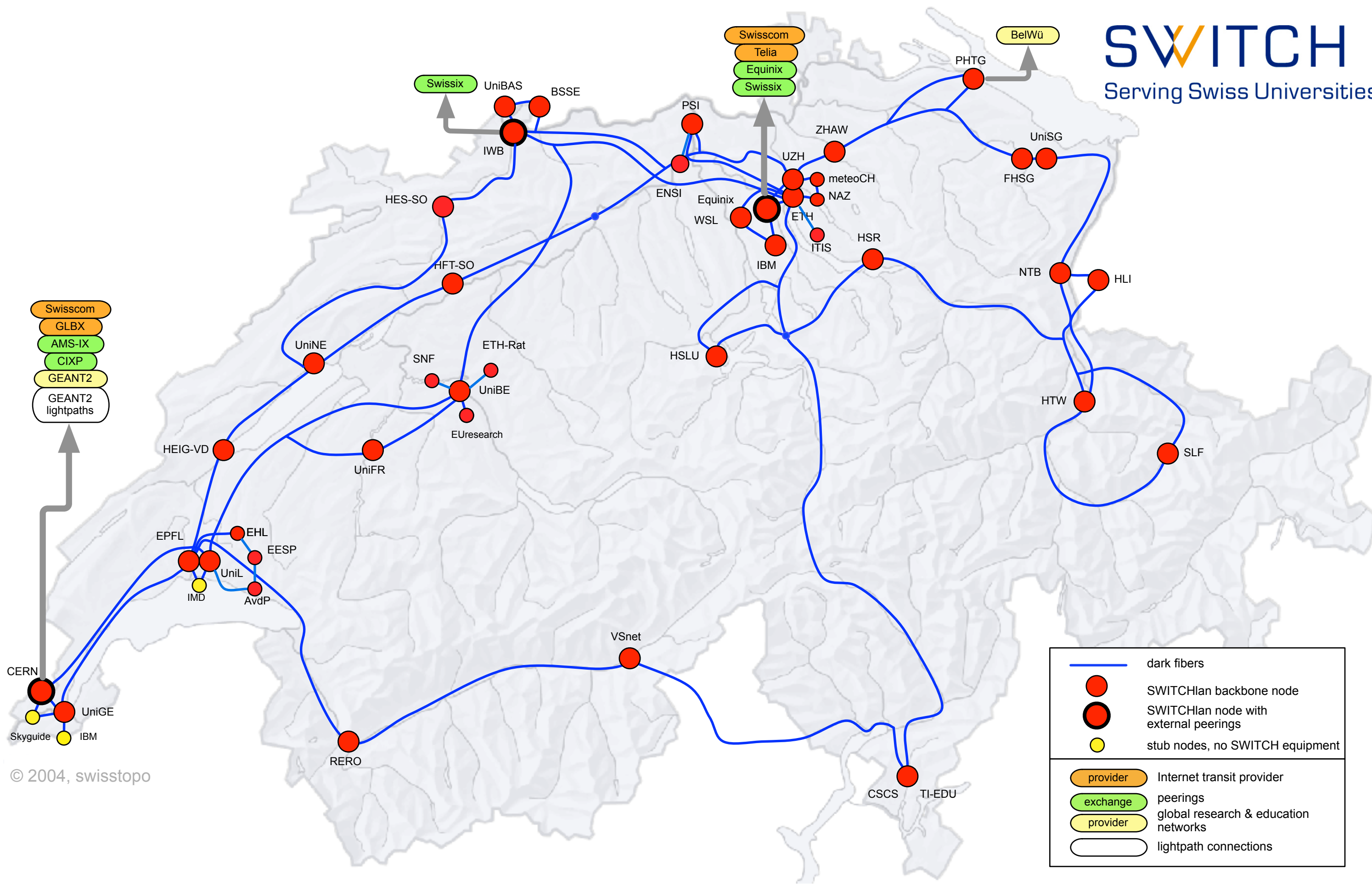
SWITCHlan Backbone: Dark Fiber Topology December 2009
